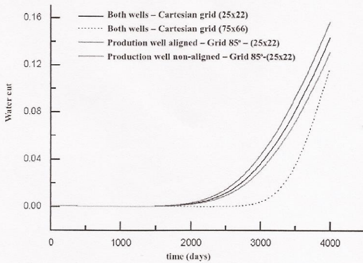
Figure 7: Water cut for the 3-well problem- 80°
