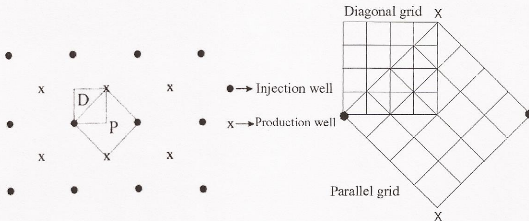
Figure 1: Five Spot Problem Configuration (a) and Cartesian Grids (b)
