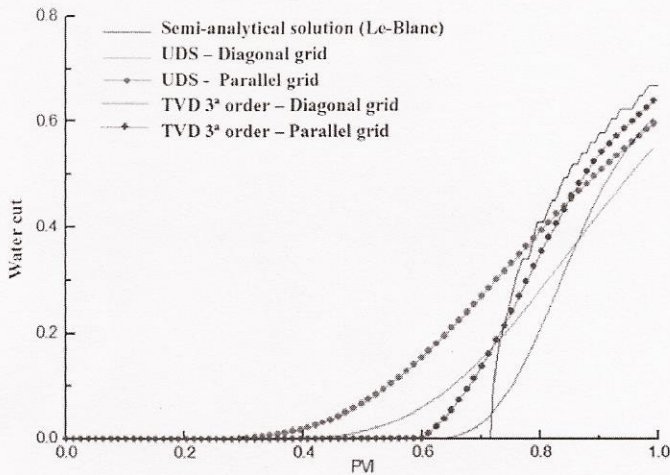
Figure 8: Five-Spot problem. UDSxTVD
