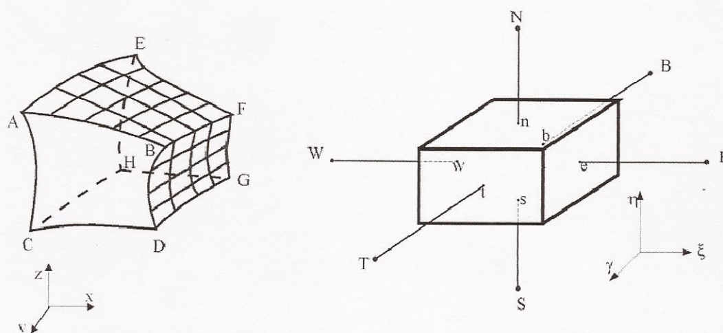
Figure 2: Physical and computational domains
